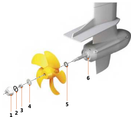
Fig. 39: Propeller attachment
