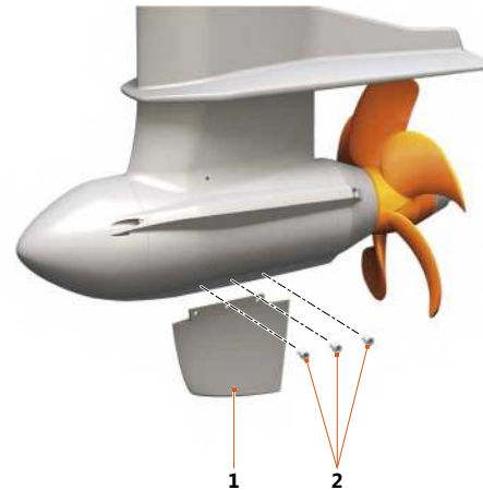
Fig. 38: Fin attachment
