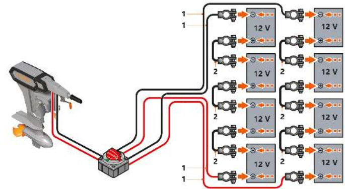
Fig. 43: Wiring diagram for lead batteries
